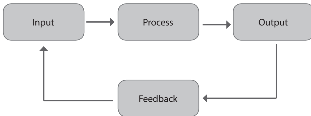
Figure 4 Open and closed loop systems
